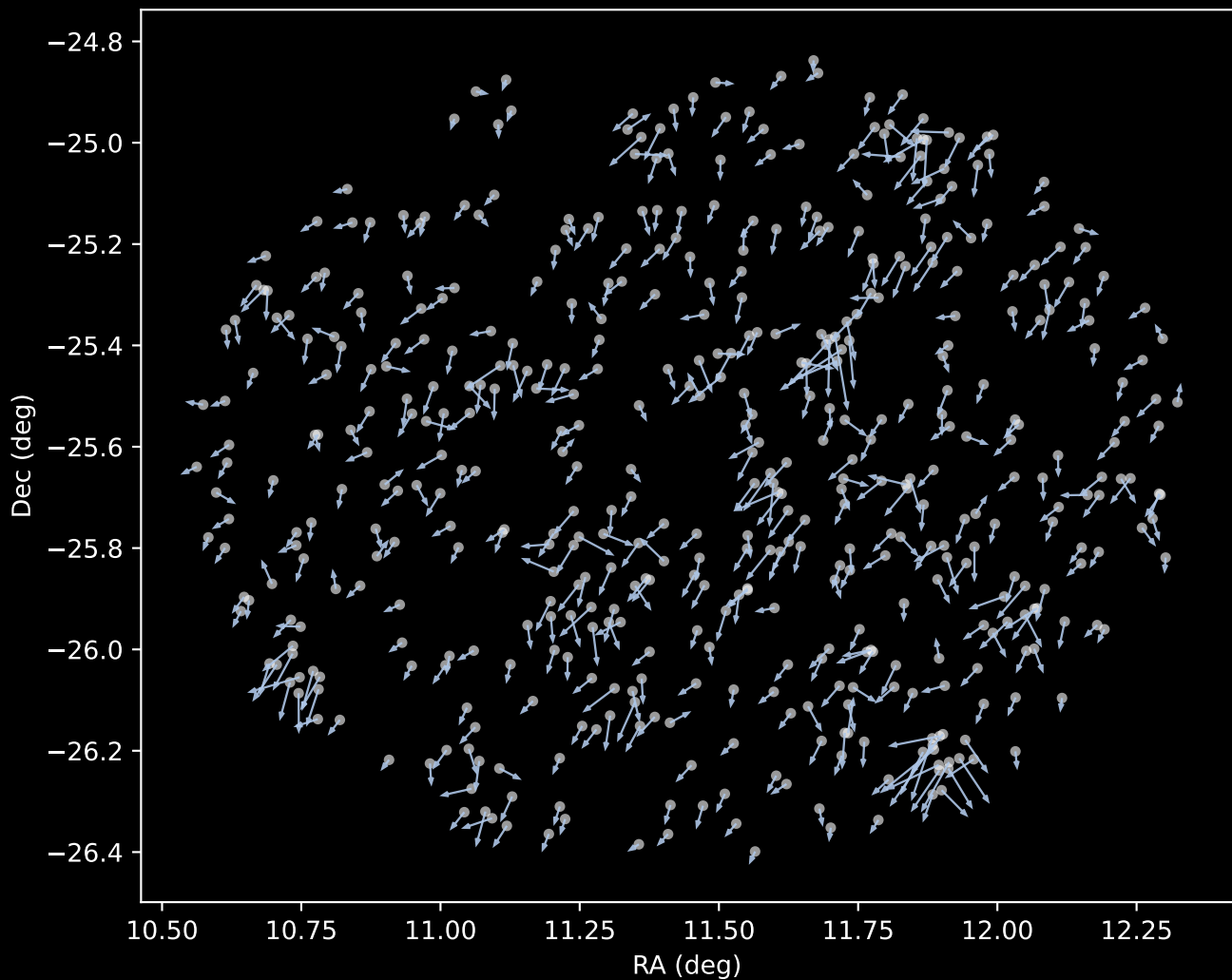
APOGEE DR17 Cluster 1 Proper Motion Vectors (n=488)
