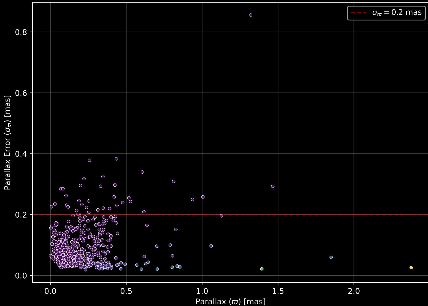
APOGEE DR17 Field: [005-02] Parallax Quality (n= 498)
