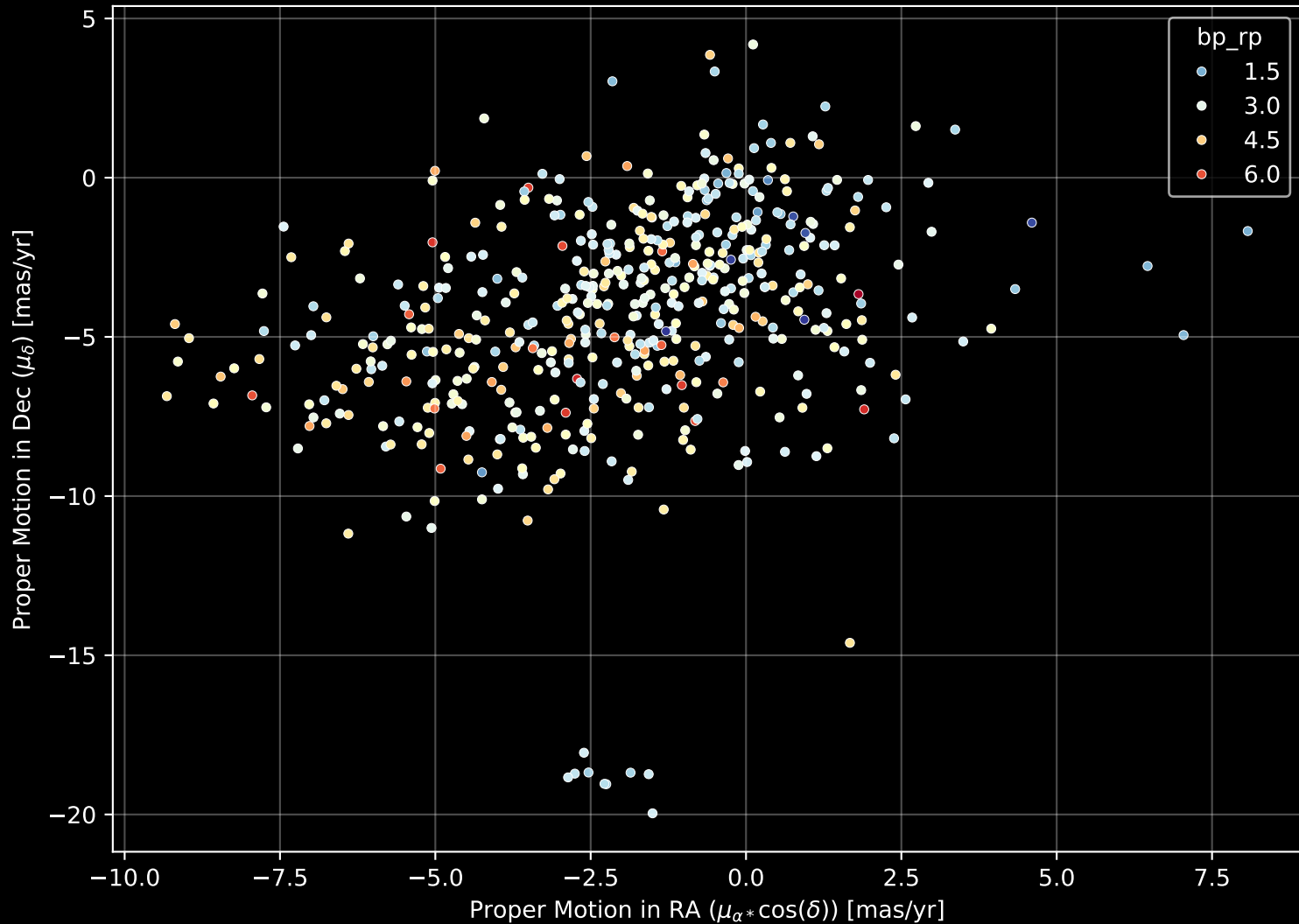
APOGEE DR17 Field: [005-02] Proper Motion Diagram (n= 498)
