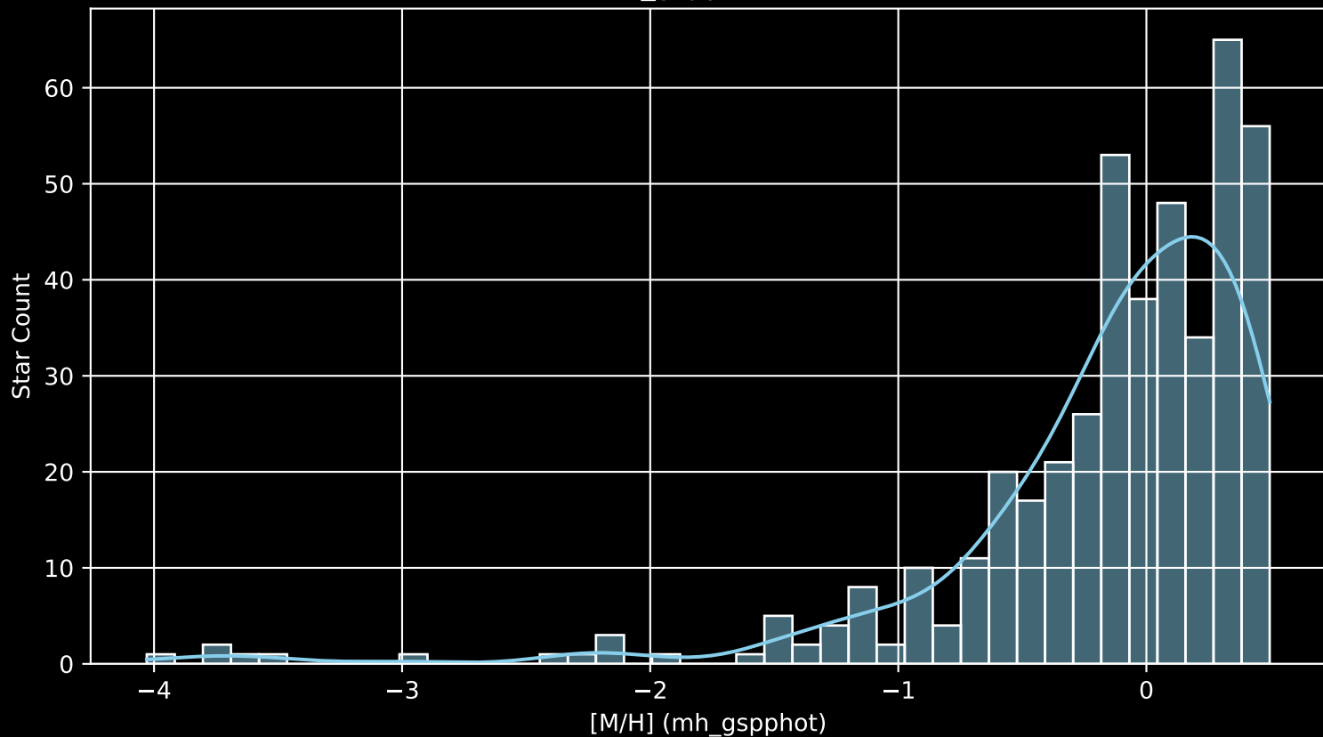
APOGEE DR17 Field: [005-02 [M/H] (mh_gspphot) (n= 437)
