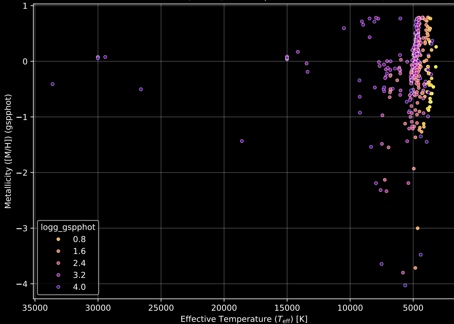
APOGEE DR17 Field: [005-02] Stellar Population Parameters (n= 498)
