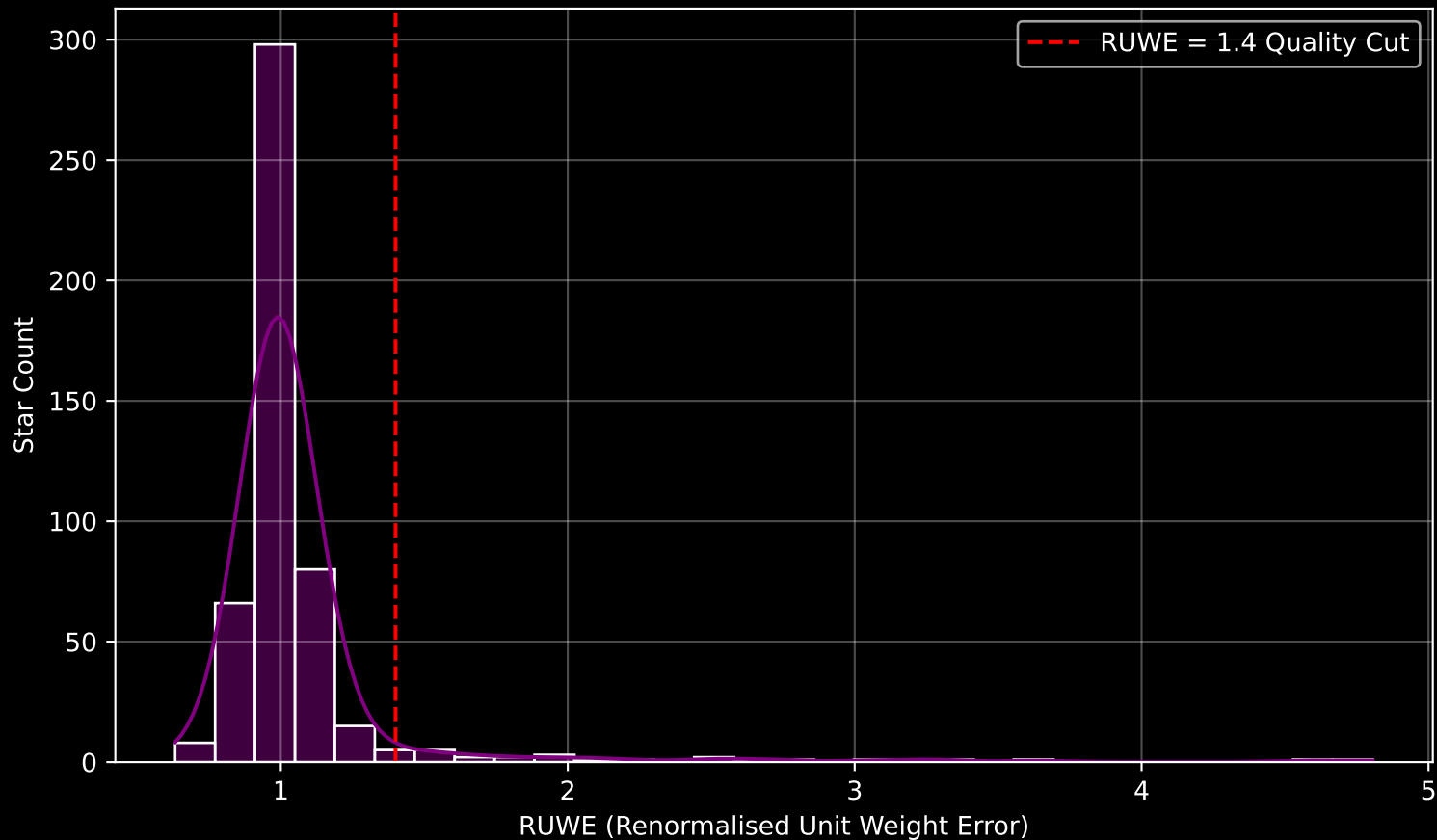
GAPOGEE DR17 Field [005-02] RUWE Distribution (n= 496)
